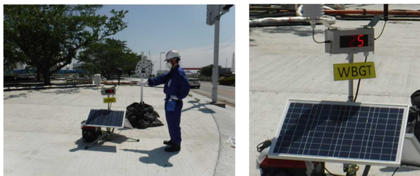
Portable WBGT display and outdoor clock (left: full view; right: enlarged display) (Fukushima Daiichi NPS)
