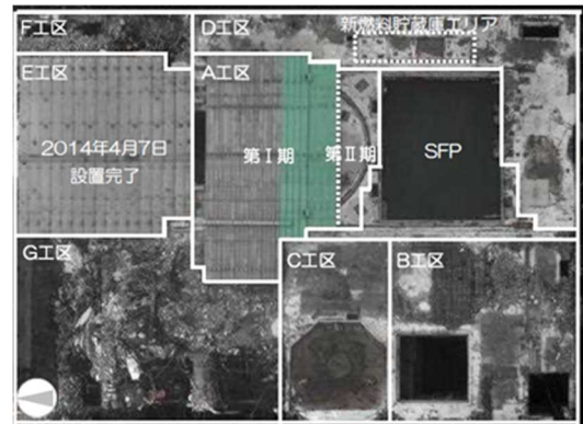
Panoramic view of Unit 3 operating floor
