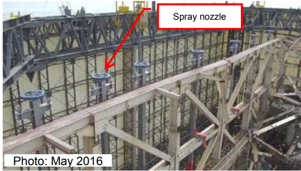
Installation of sprinkler system nozzle units
