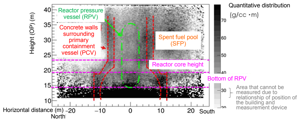
Assessment of quantitative distribution based on measurements taken using the muon transmission method
