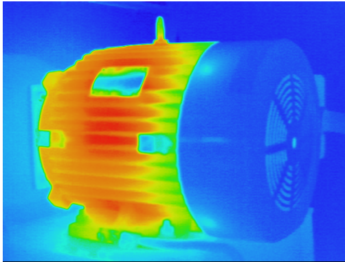
Data collection directly implemented by operators (Infrared thermography diagnosis of a motor)
