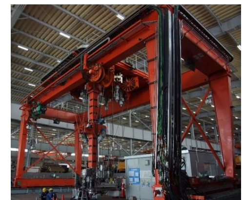
Unit 3 fuel handling machine
