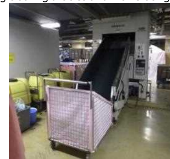
Prior to kaizen (Left: Large washing machines; Right: Large dryers)
