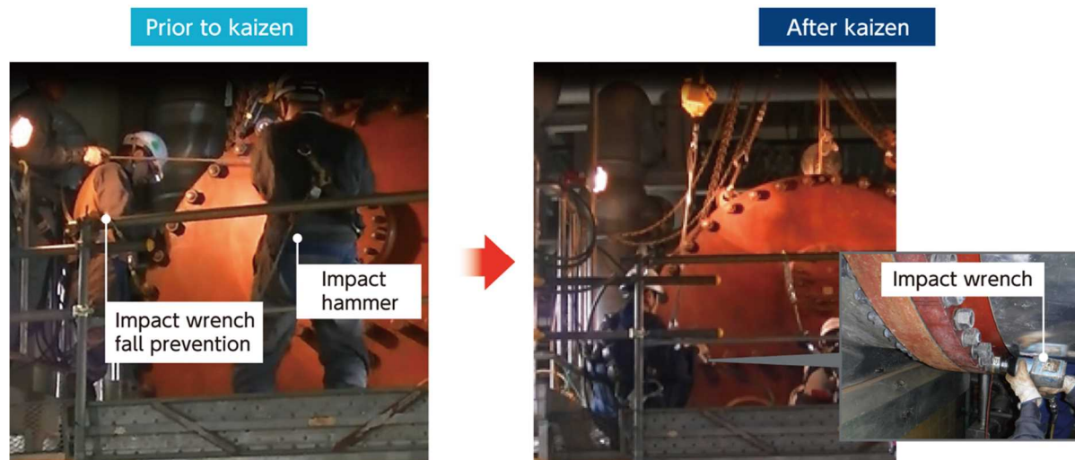
Kaizen for the removal and tightening of water chamber bolts/nuts
