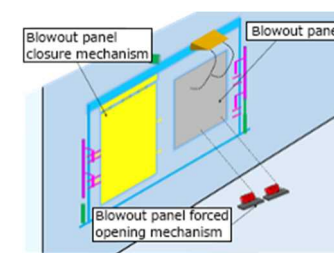
Blowout panel closure mechanism overview
